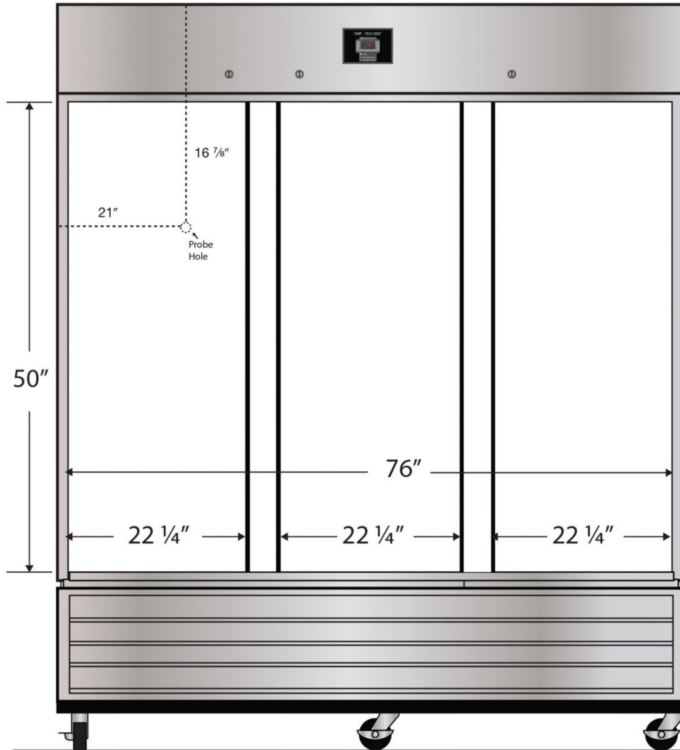
Front View
