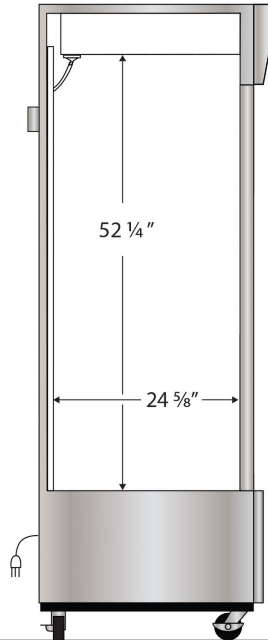
Side View
