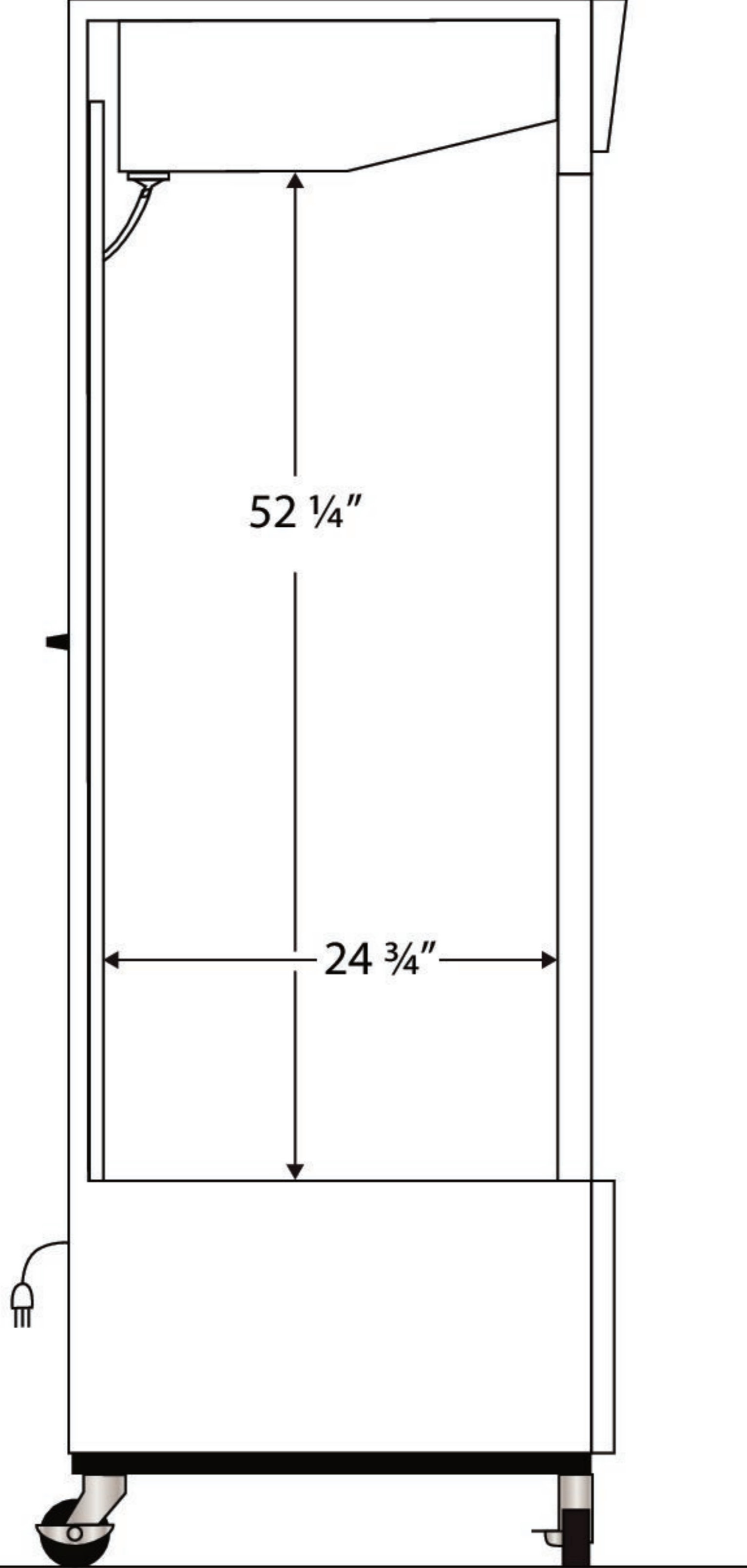
Side View
