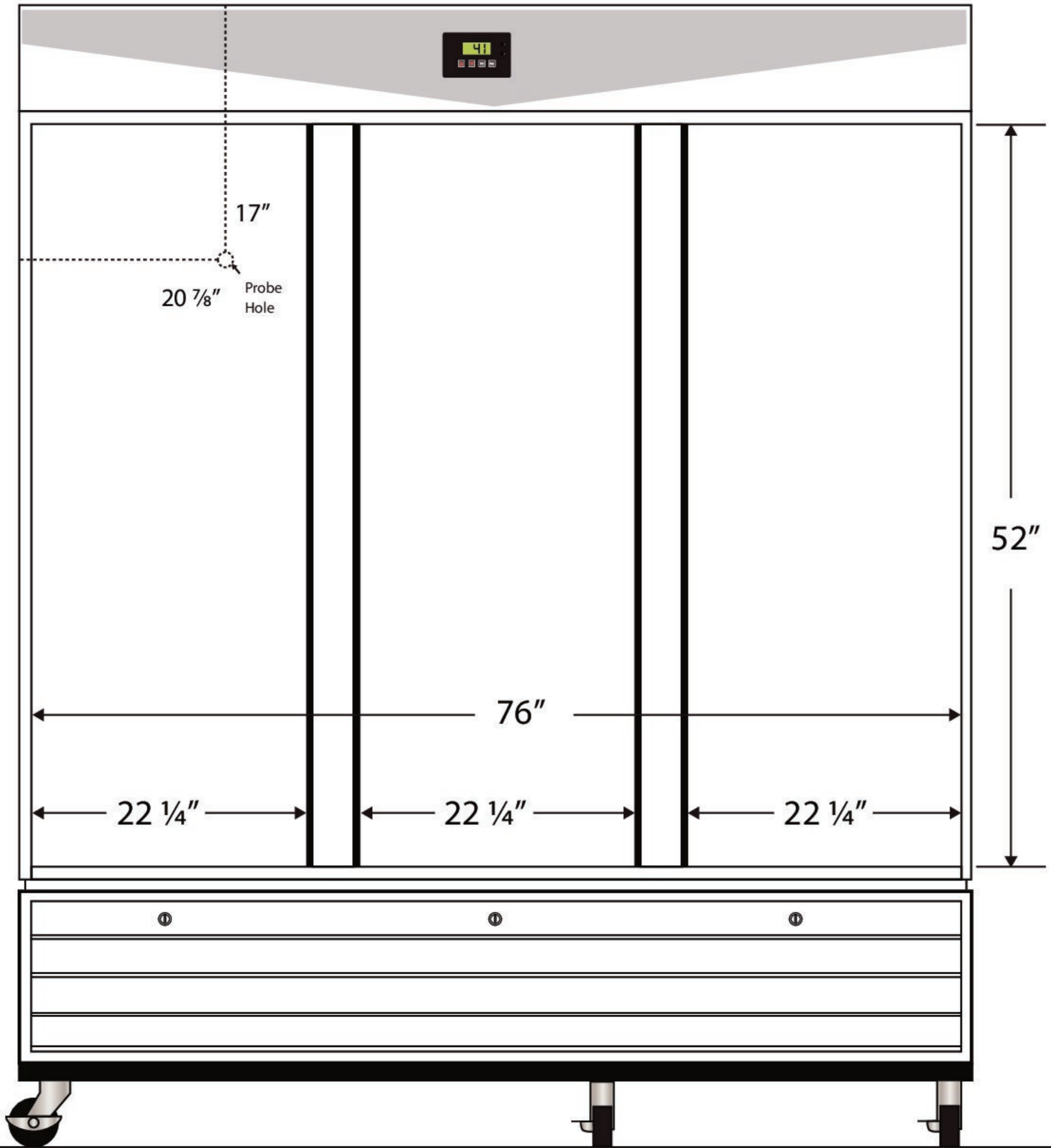
Front View
