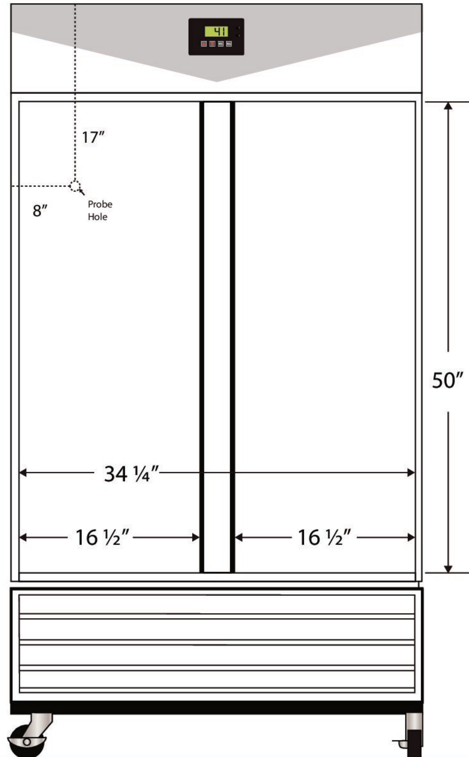
Front View
