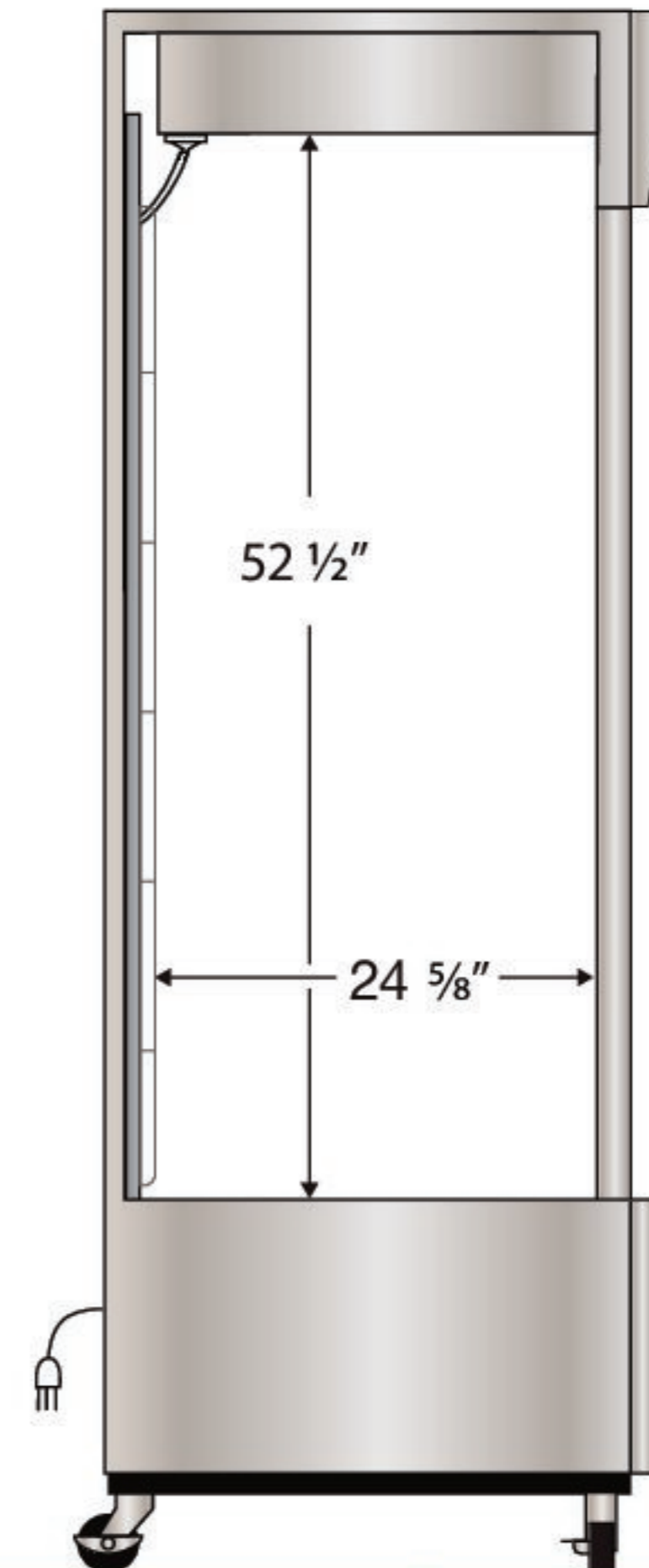
Side View
