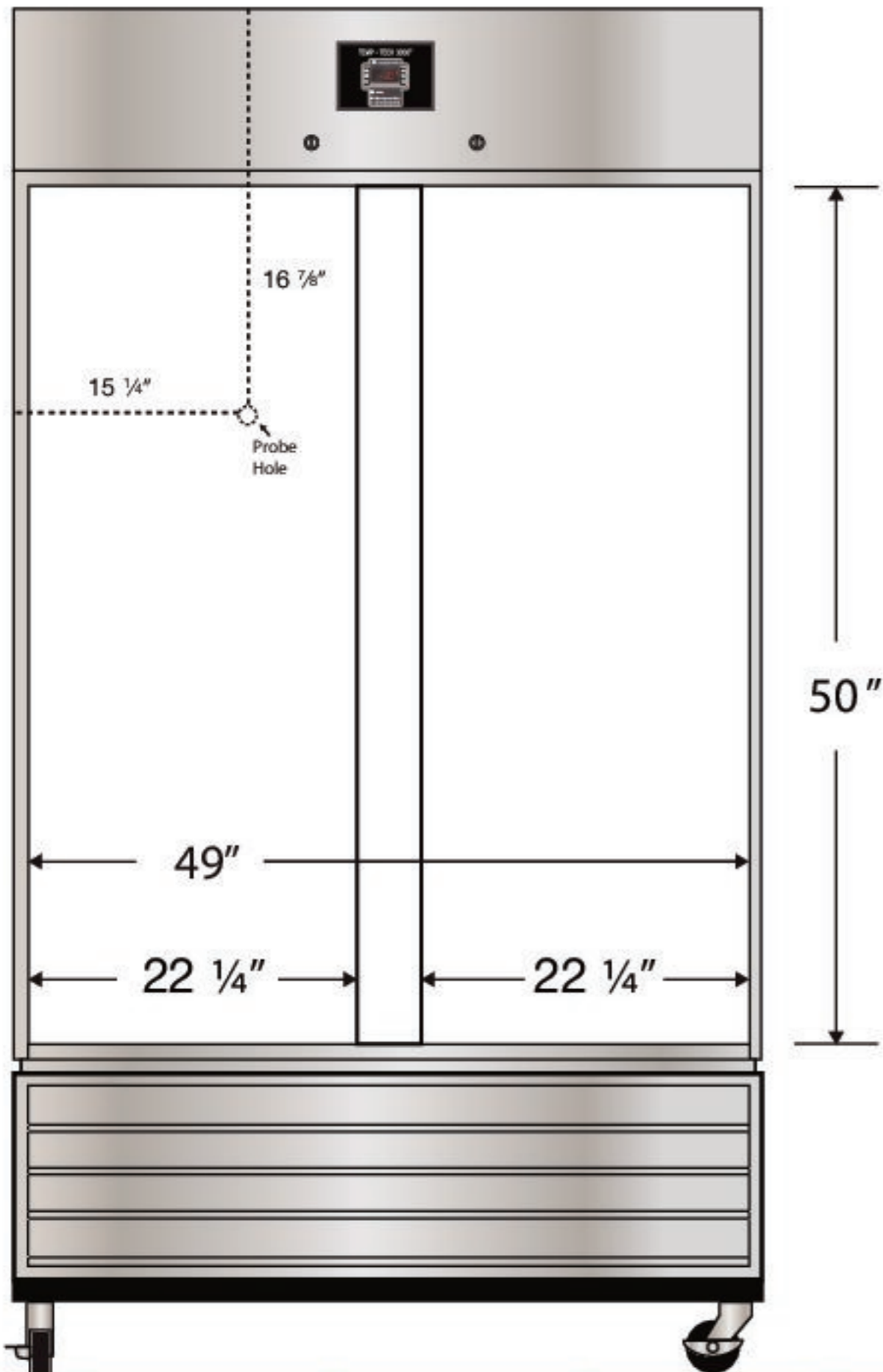
Front View
